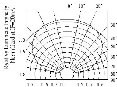
FIG.4 RADIATION DIAGRAM
